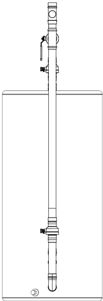
FRONT VIEW
