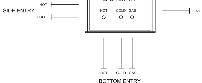
Figure 2: Piping options.
